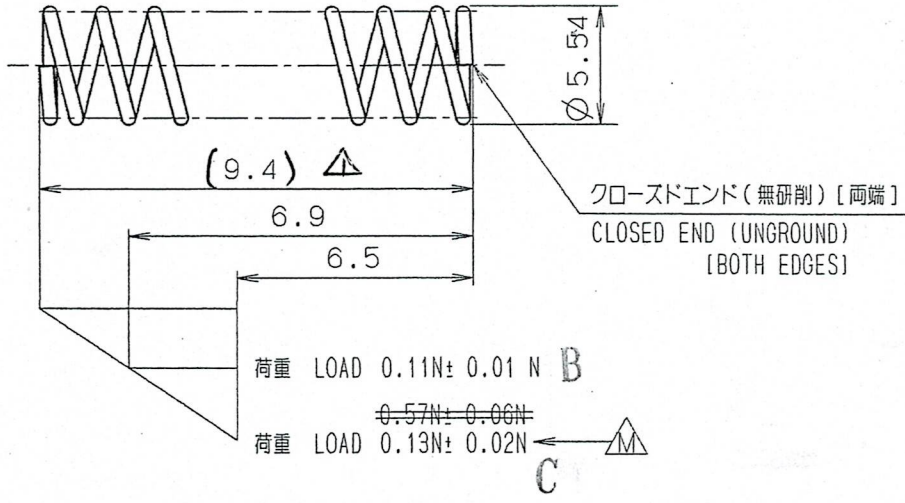
円筒圧縮コイルばね要目表 TABLE OF ESSENTIALS FOR CYLINDRICALLY COILED COMPRESSION SPRING
