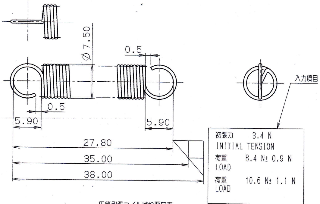
円筒引張コイルばね要目表 TABLE OF ESSENTIALS FOR CYLINDRICALLY COILED EXTENSION SPRING
